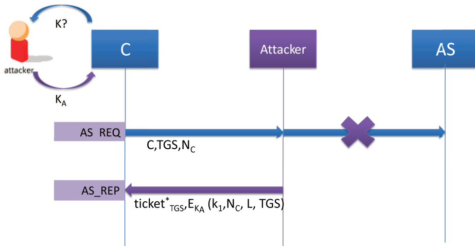
Figure 2: KDC Spoofing
