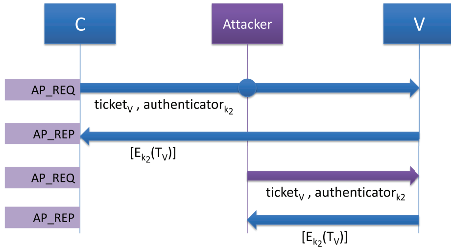
Figure 3: Replay Attack
