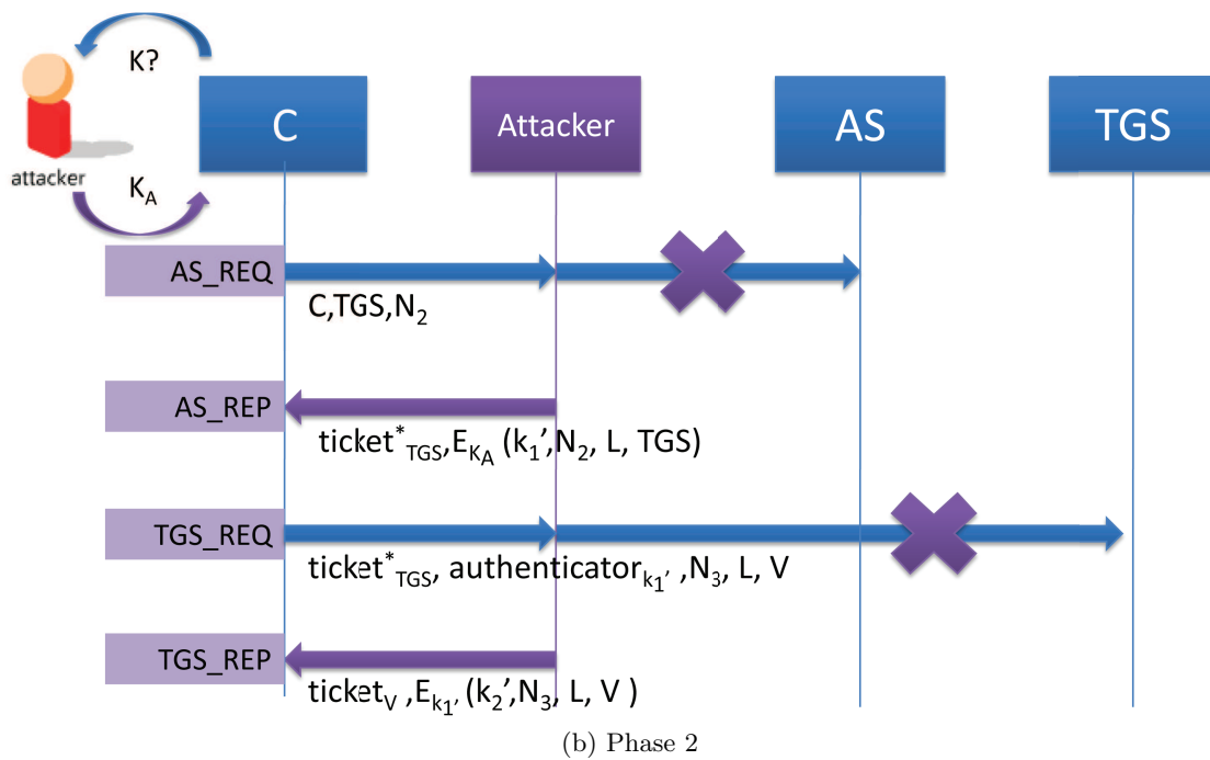
Figure 4: Pass-the-ticket attack
