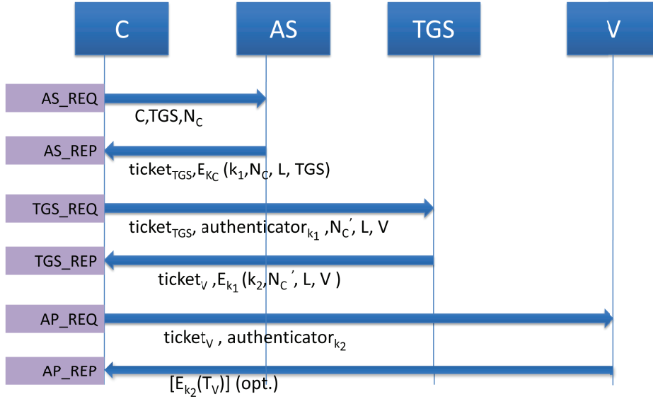
Figure 1: The Kerberos V protocol
